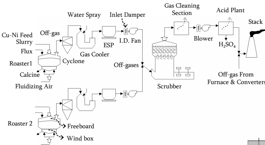
Schematic Diagram of Roaster Off-gas System
